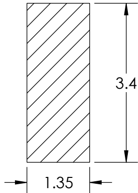
SECTION E-E SCALE 1 : 2
